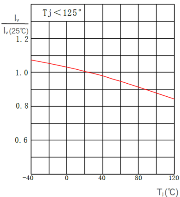
相对发光强度 / Relative Luminous Intensity I_v/I_v(25^\circ\text{C}) = f(T_j); I_f = 20\text{ mA}
