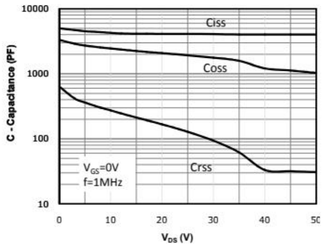
Fig 6: Capacitance Characteristics
