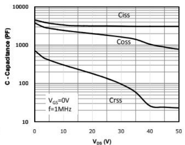
Fig 6: Capacitance Characteristics
