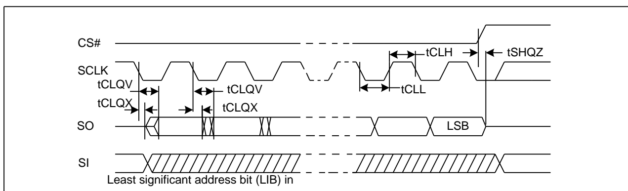
Figure 40. Output Timing
