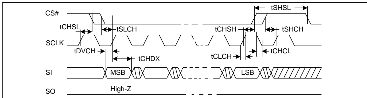
Figure 39. Serial Input Timing
