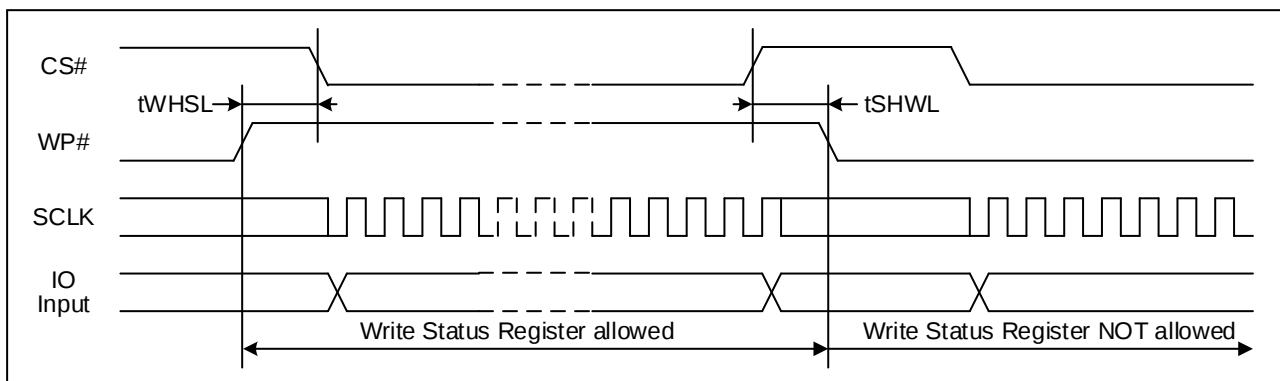
Figure 42. WP# Timing
