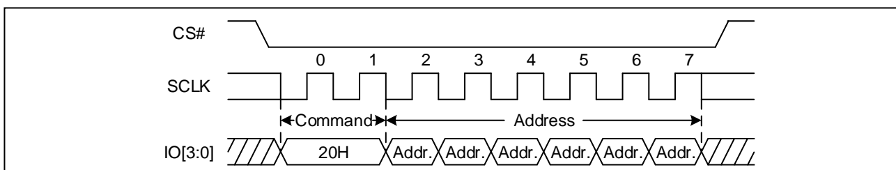
Figure 29. Sector Erase Sequence Diagram (QPI)
