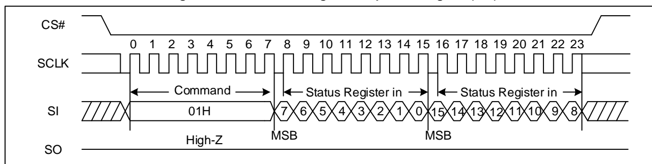
Figure 10. Write Status Register Sequence Diagram (SPI)
