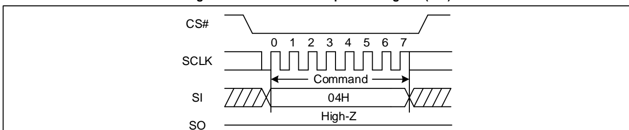
Figure 6. Write Disable Sequence Diagram (SPI)
