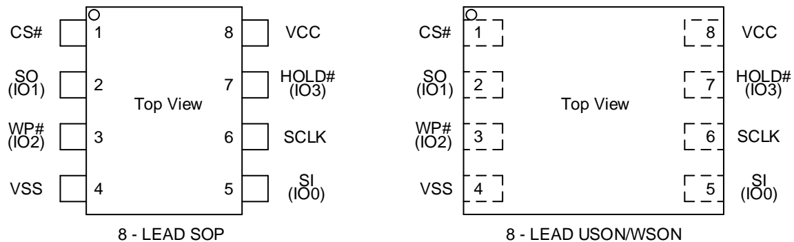
Figure 1 Connection Diagram for SOP8/USON8/WSN8 package
