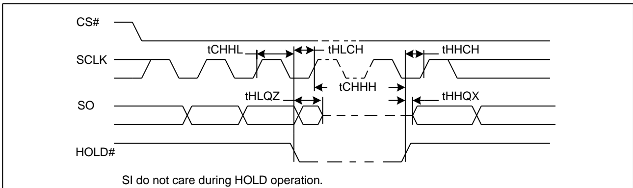
Figure 68. Hold Timing
