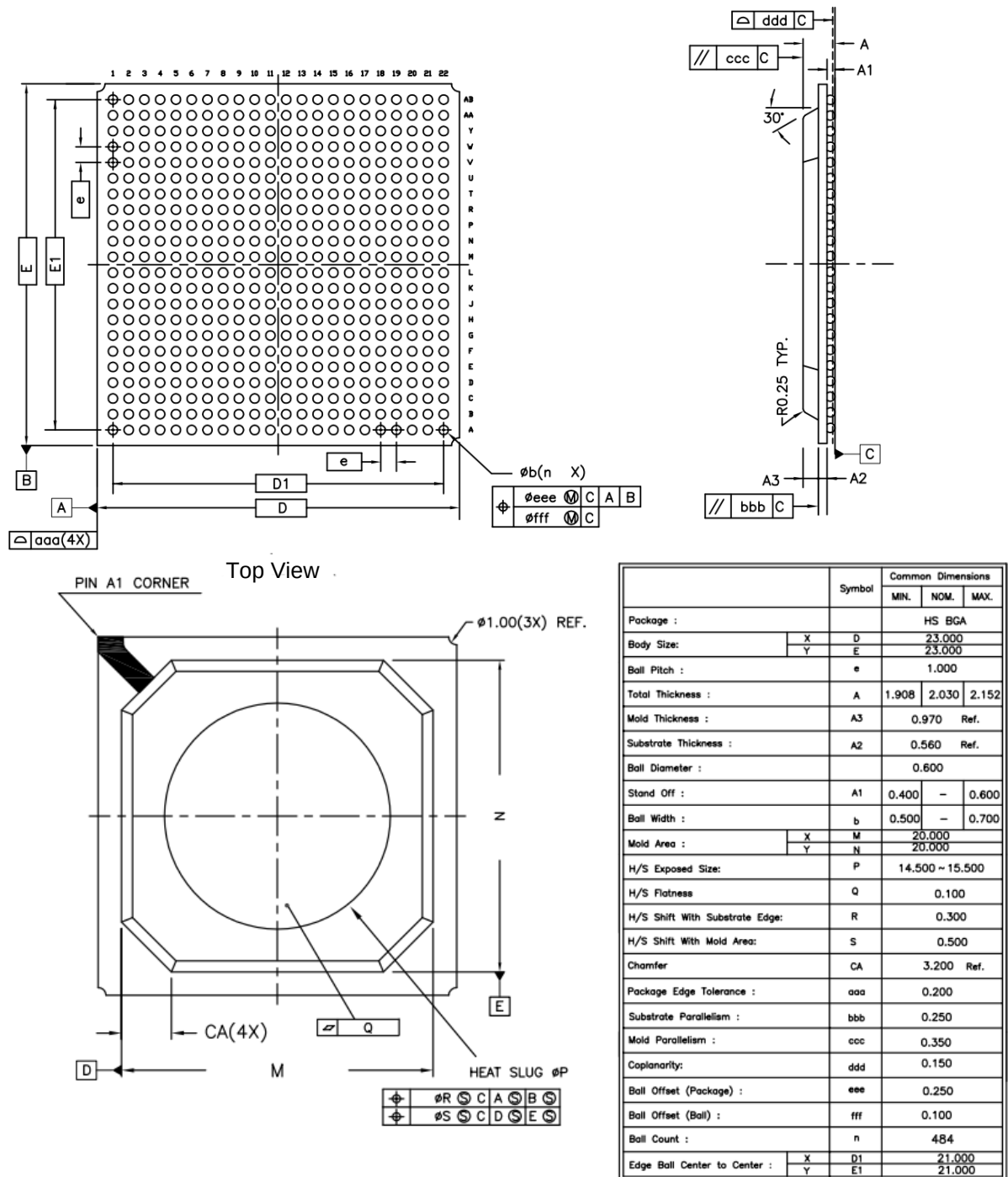
Figure 16: VS2010RX Mechanical Information (all dimensions in mm)
