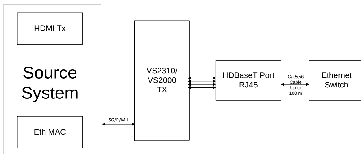
Figure 17: VS2310TX/VS2000TX in Ethernet Fallback Mode
