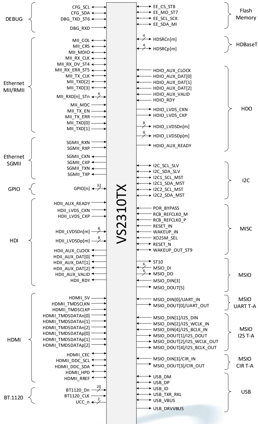
Figure 7: VS2310TX I/F Signal Block Diagram
