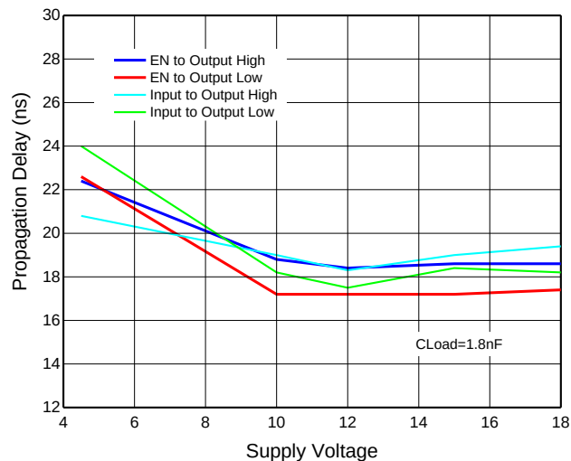
Figure 22. Propagation Delay vs Supply Voltage
