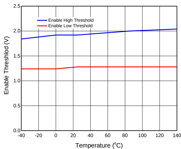
Figure 14. Enable Threshold vs Temperature
