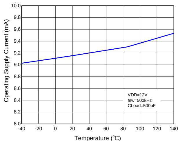
Figure 10. Operating Supply Current vs Temperature
