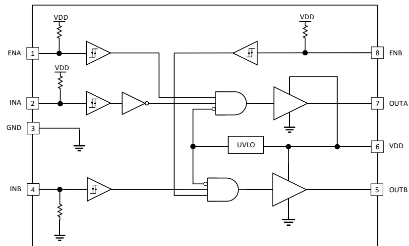
Figure 4. SLM27525 Block Diagram
