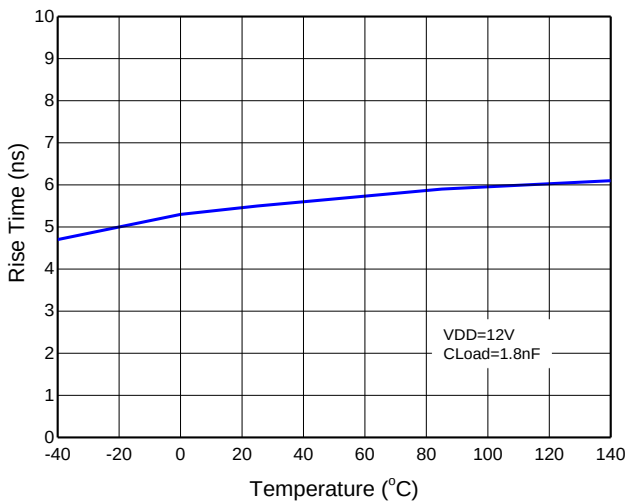
Figure 17. Rise Time vs Temperature
