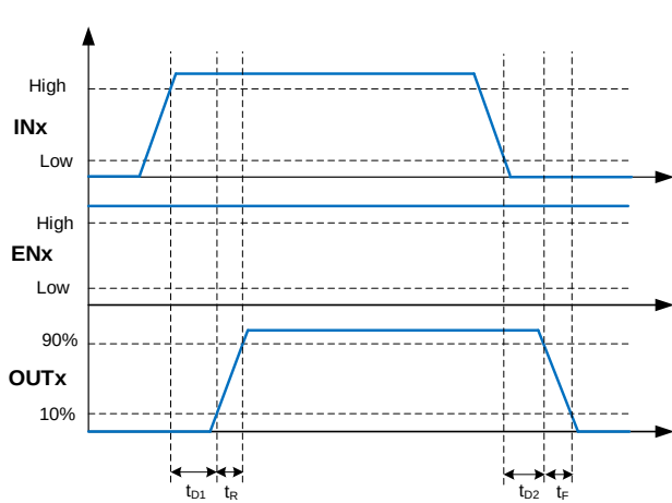
Figure 7. Non-Inverting Input Driver Operation
