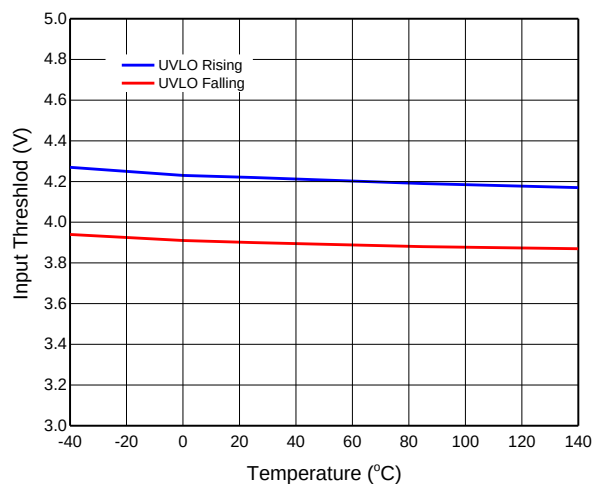
Figure 12. UVLO Threshold vs Temperature
