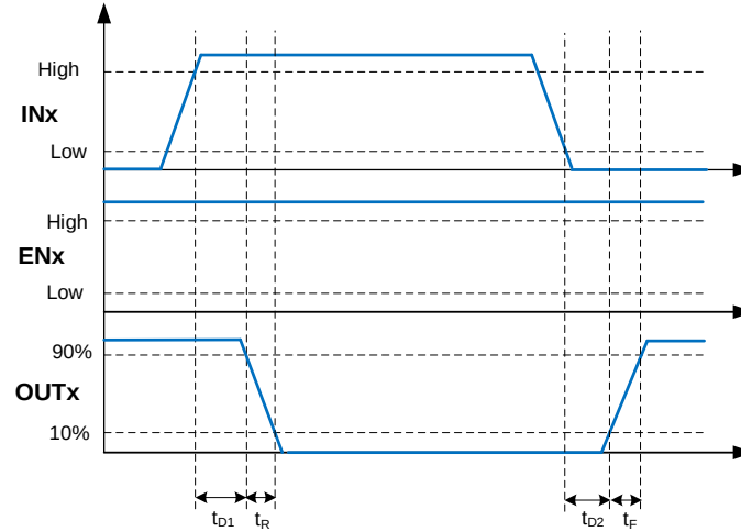
Figure 8. Inverting Input Driver Operation
