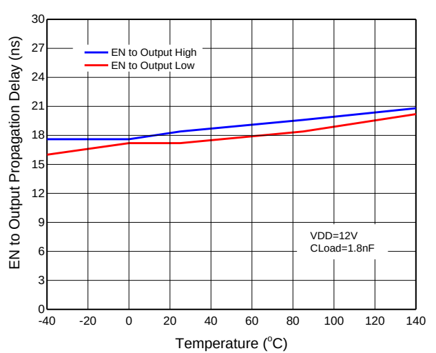
Figure 20. Enable to Output Propagation Delay vs Temperature
