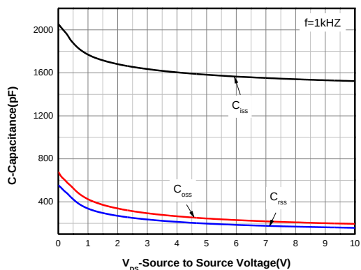
Capacitance
