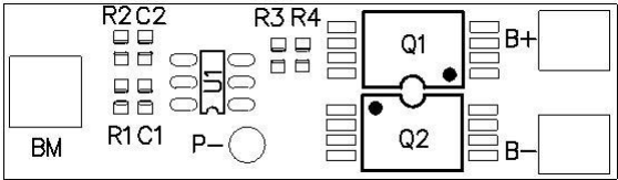
TOP SILKSCREEN
