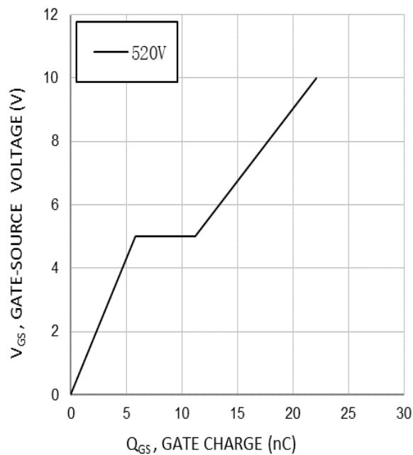
Fig.2 Gate Charge
