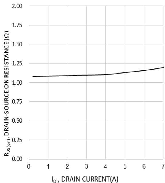
Fig.6 Drain-Source On Resistance
