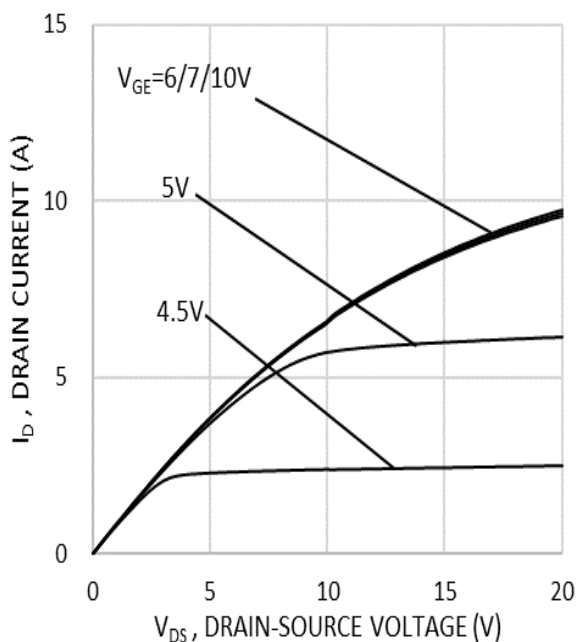
Fig.5 Output Characteristics
