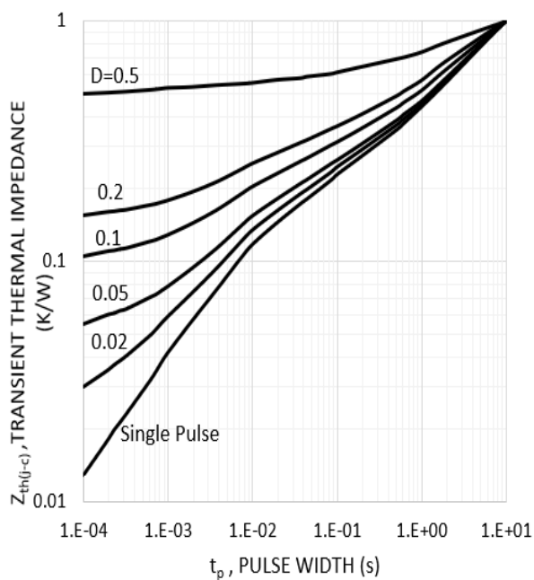
Fig.4 Thermal Transient Impedance
