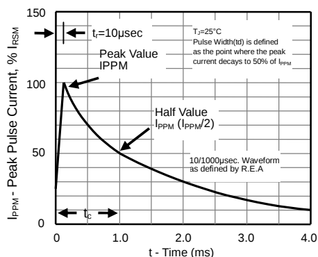
Figure 3 -Pulse Waveform
