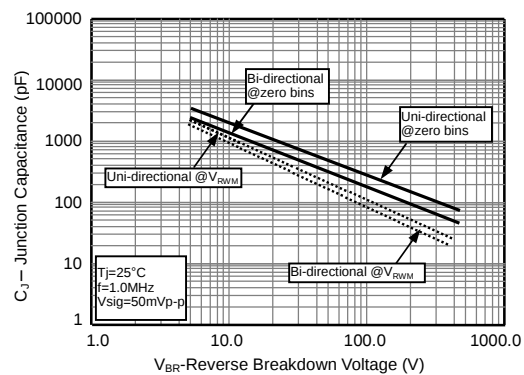
Figure 4 -TypicalJunction Capacitance
