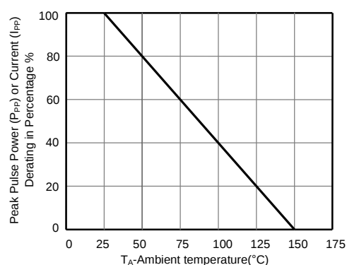
Figure 2 -Pulse DeratingCurve
