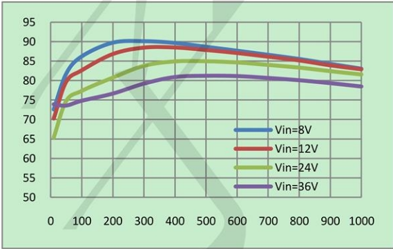
Efficient @Vout=3.3V
