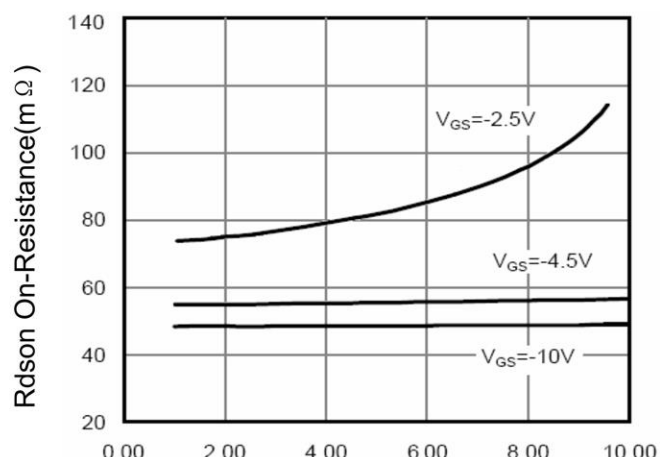
Figure 6 Drain-Source On-Resistance
