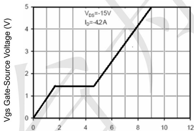
Figure 11 Gate Charge
