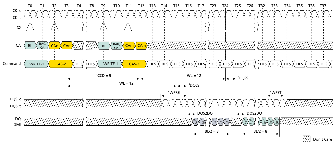
Figure 56: Consecutive WRITE: t_{CCD} = \text{MIN} + 1, 1.5n\text{CK} Postamble
