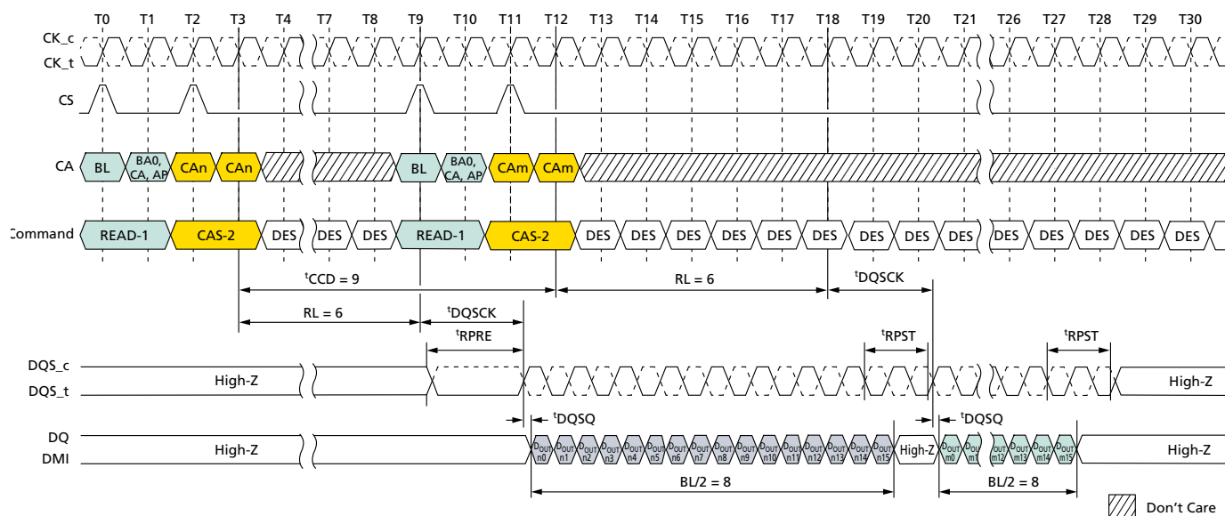
Figure 42: Consecutive READ: t_{CCD} = \text{MIN} + 1 , Preamble = Static, 1.5n\text{CK} Postamble
