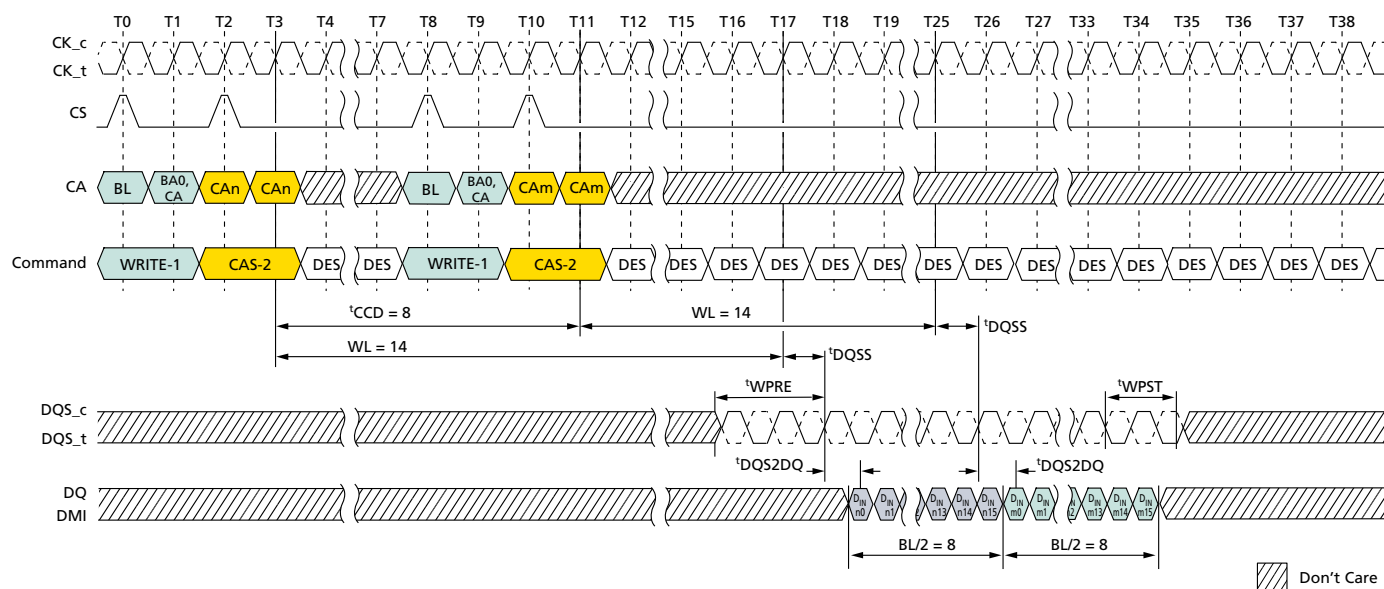
Figure 54: Seamless WRITE: t_{\text{CCD}} = \text{MIN} , 1.5n\text{CK} Postamble
