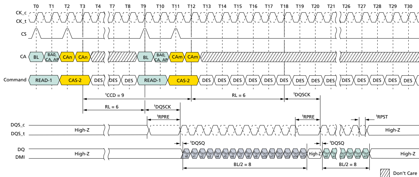
Figure 43: Consecutive READ: t_{CCD} = \text{MIN} + 1 , Preamble = Static, 0.5n\text{CK} Postamble
