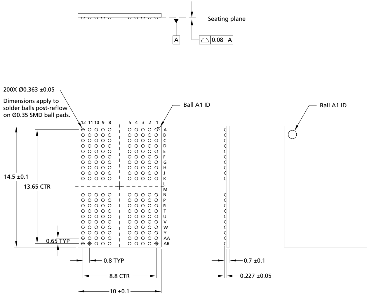
Figure 6: 200-Ball WFBGA – 10mm x 14.5mm x 0.8mm (Package Code: DS)
