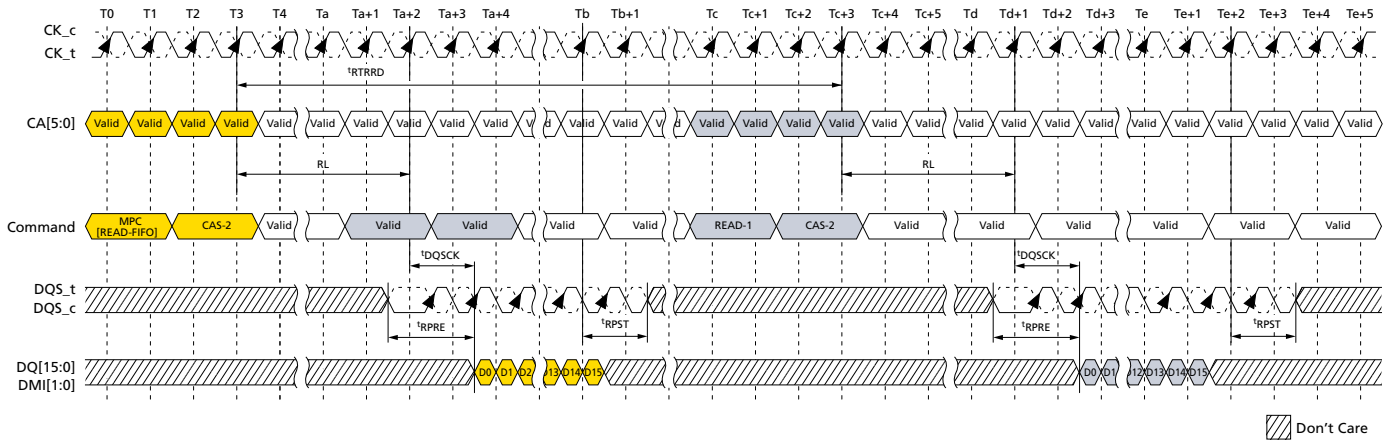
Figure 122: READ-FIFO – t_{\text{RPRE}} = \text{Toggle} , t_{\text{RPST}} = 1.5n\text{CK}
