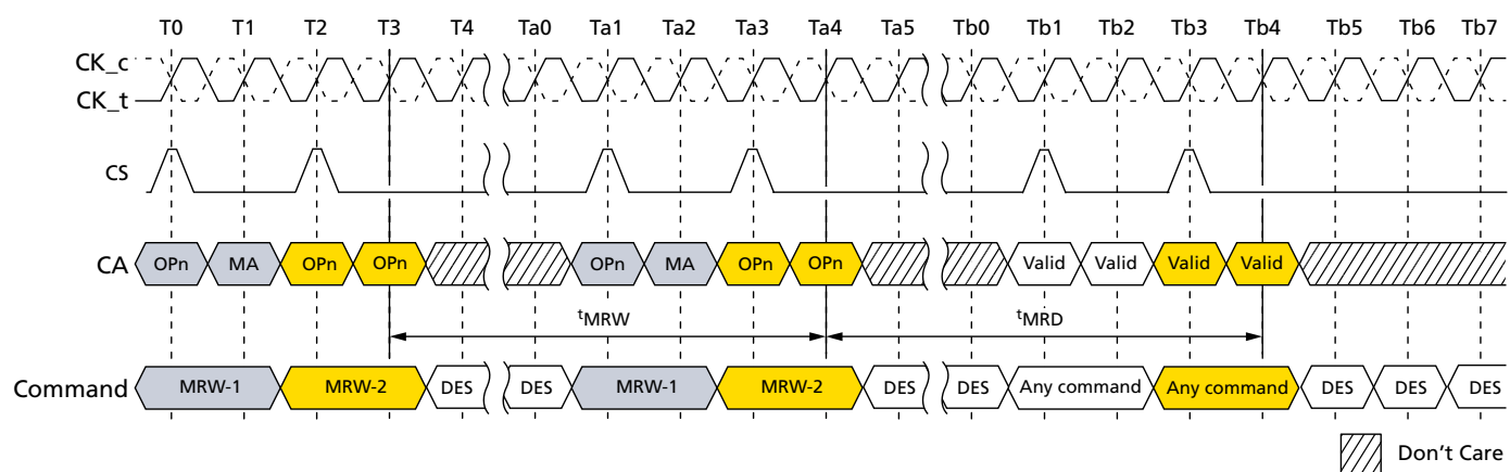
Figure 95: MODE REGISTER WRITE Timing
