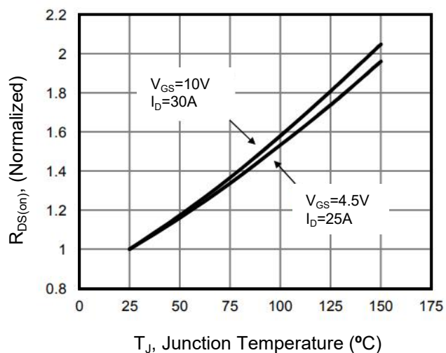
Figure 7. Drain-Source On-Resistance
