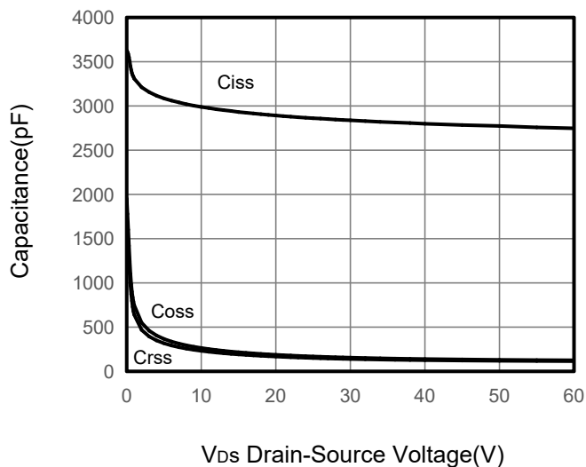
Figure 5. Capacitance
