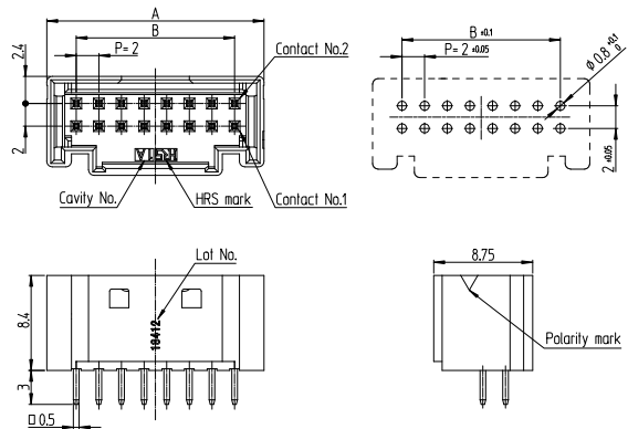
Recommended PCB Layout (t=1.6mm)
