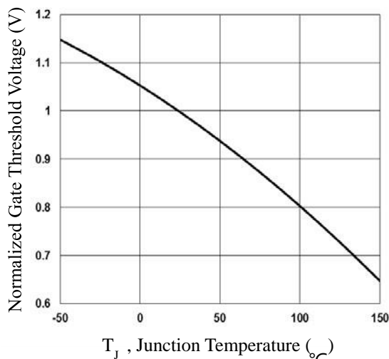
Fig.3 Normalized Vth vs. Tj J
