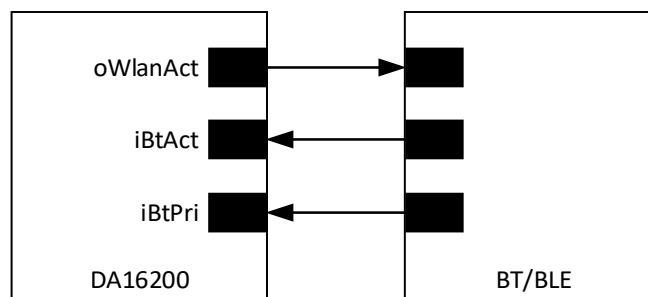
Figure 57: Bluetooth Coexistence Interface
