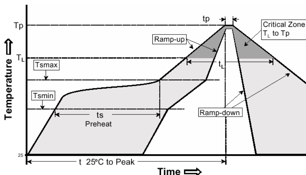
Figure 78: Reflow Condition
