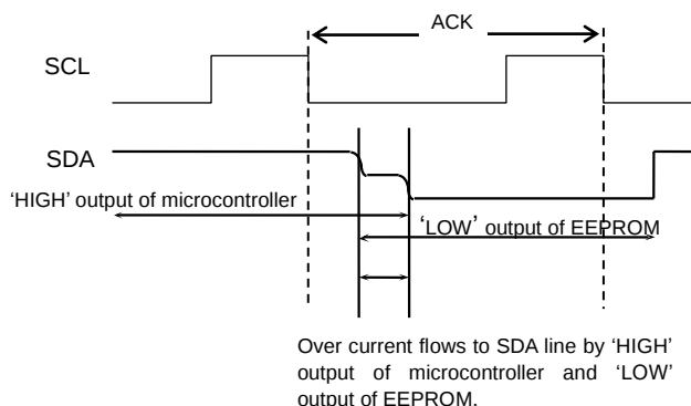
Figure 53. I/O Collision Timing
