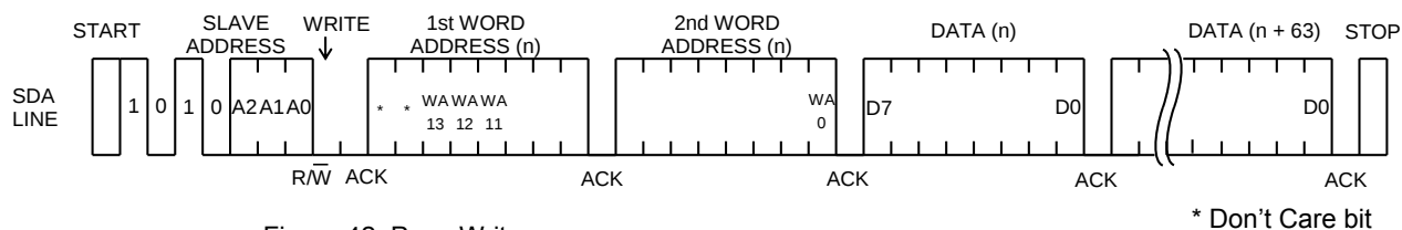
Figure 42. Page Write
