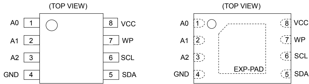
Figure 3-(a). Pin Configuration (SOP8, SOP-J8, TSSOP-B8, MSOP8)
