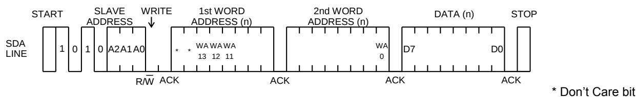
Figure 41. Byte Write
