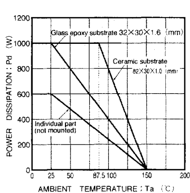
Fig. 1 Derating curve
