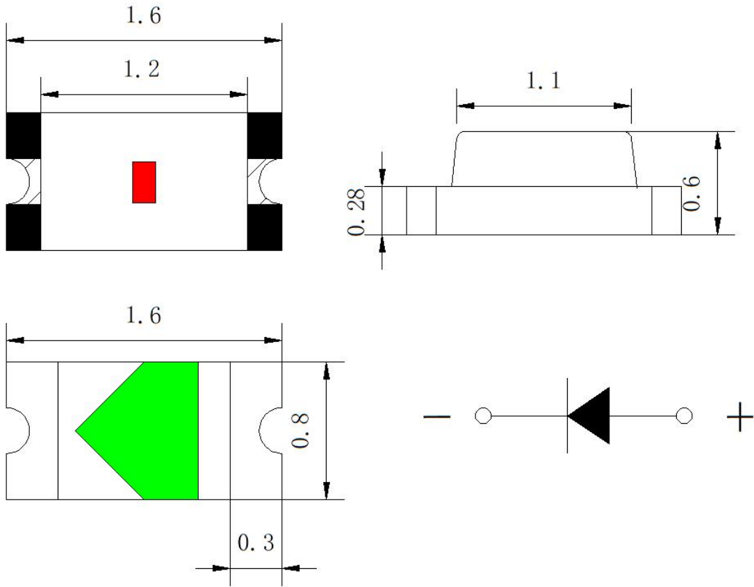
Recommended Solder Pad Design 推荐焊盘设计
