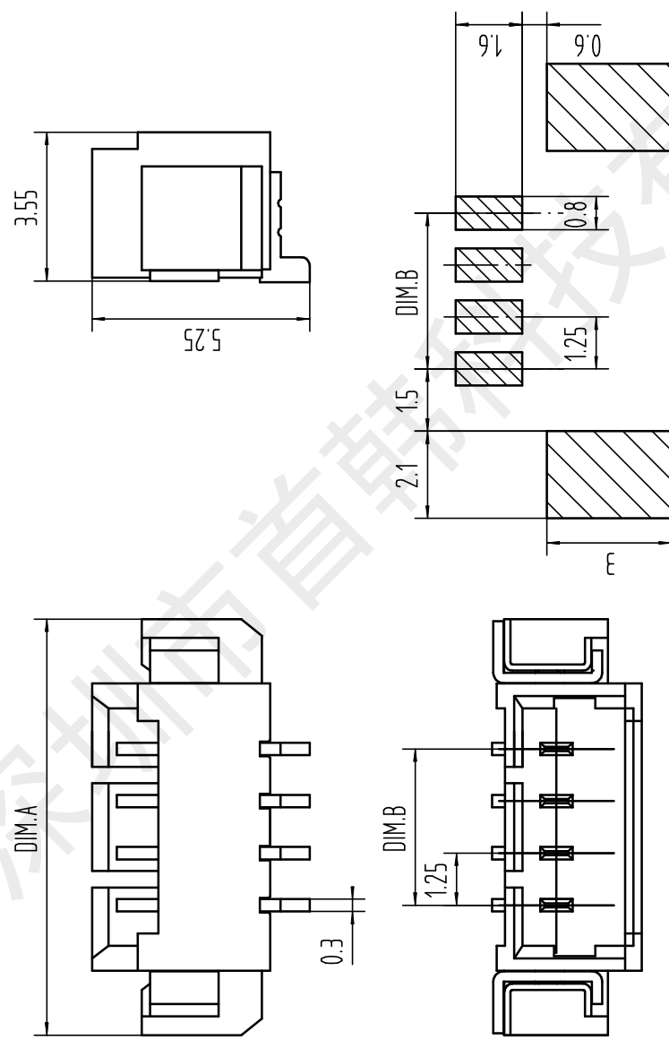
PCB LAYOUT
