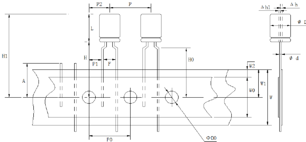
[ Fig. 1 (Diameter for Φ4 to Φ8)]
