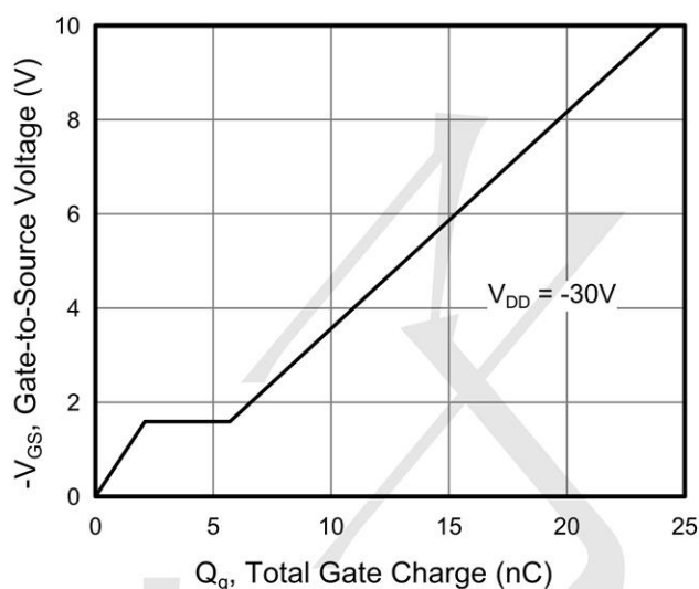
Figure 8. Gate Charge
