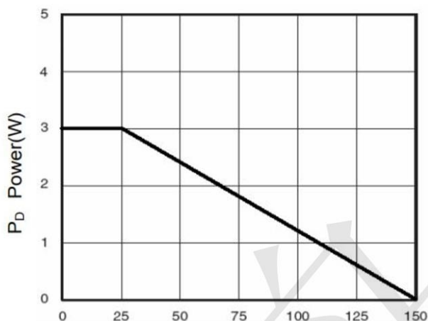
Figure 3 Power Dissipation
