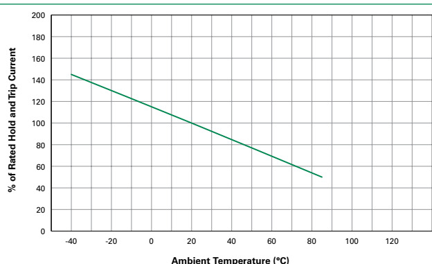
Temperature Rerating Curve
