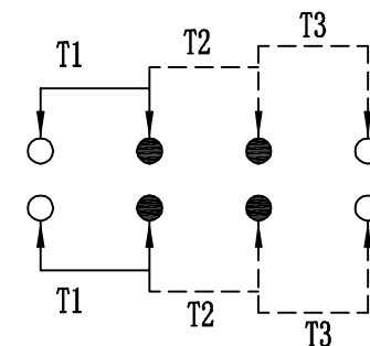
SCHEMATIC (NON-SHORTING)
