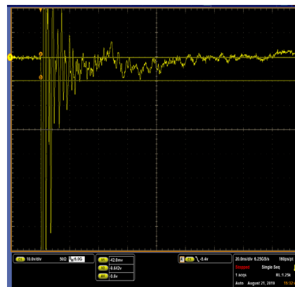
IEC 61000-4-2 -8kV Contact ESD Clamping Voltage
