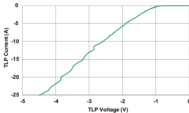
Negative Transmission Line Pulsing (TLP) Plot
