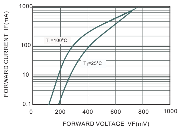
Fig.3 Forward Characteristics
