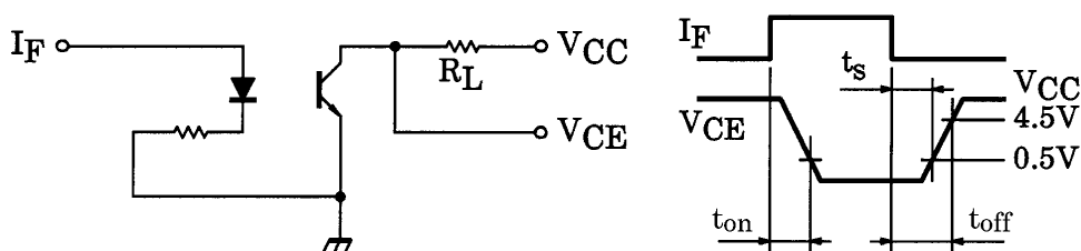
Fig. 10.1 Switching Time Test Circuit and Waveform
