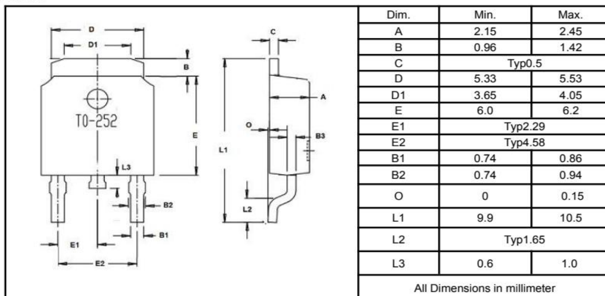
TO-252
