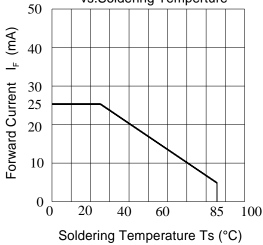
Fig.5-Max.Driving Forward Current vs.Soldering Temperpurture
