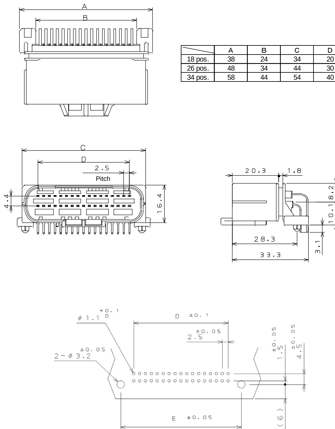
Recommended foot-pattern for PWB (reference)
