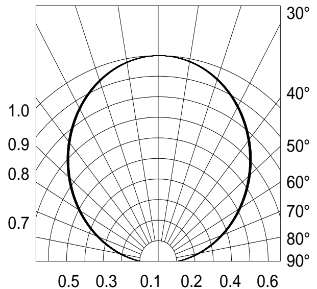
Fig.6-Radiation Diagram Ta=25°C
