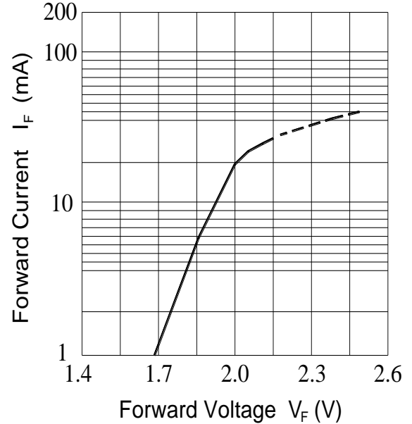
Fig.4-Forward Current vs. Forward Voltage Ta=25°C
