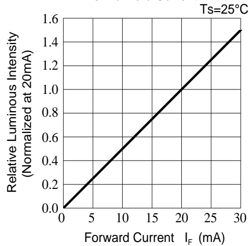
Fig.2-Relative Luminous Intensity vs. Forward Current Ts=25°C
