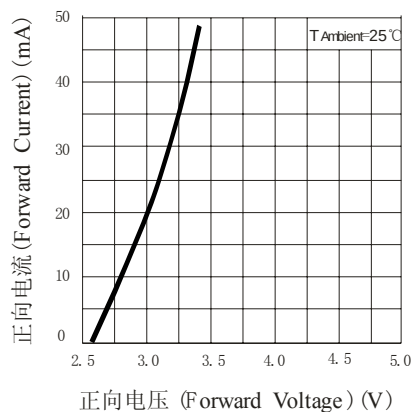
Volt-Ampere Characteristics
