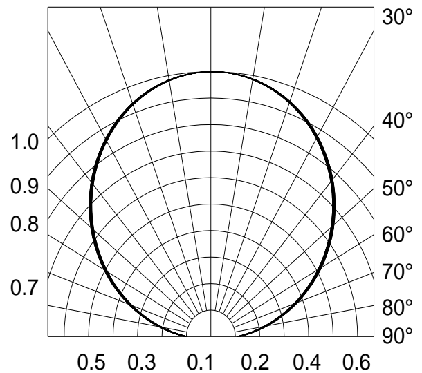
Fig.6-Radiation Diagram T_a=25^\circ\text{C}
