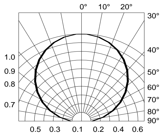
Fig.6-Radiation Diagram Ta=25°C
