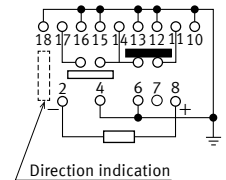
1 coil latching (Reset)
