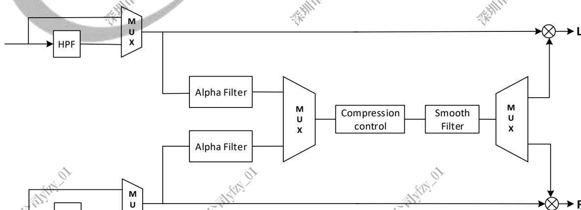
Figure 8-17 DAP Data Flow
