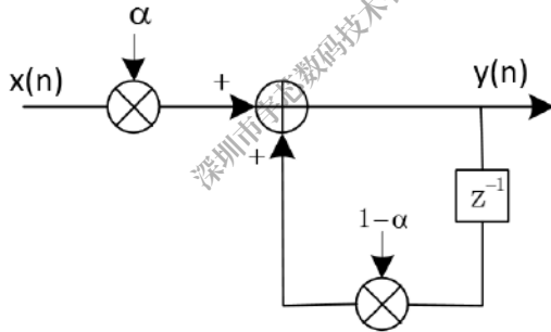
Figure 8-21 Energy Filter Structure
