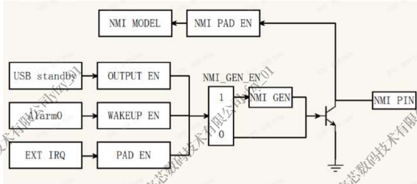
Figure 3-46 NMI Block Diagram
