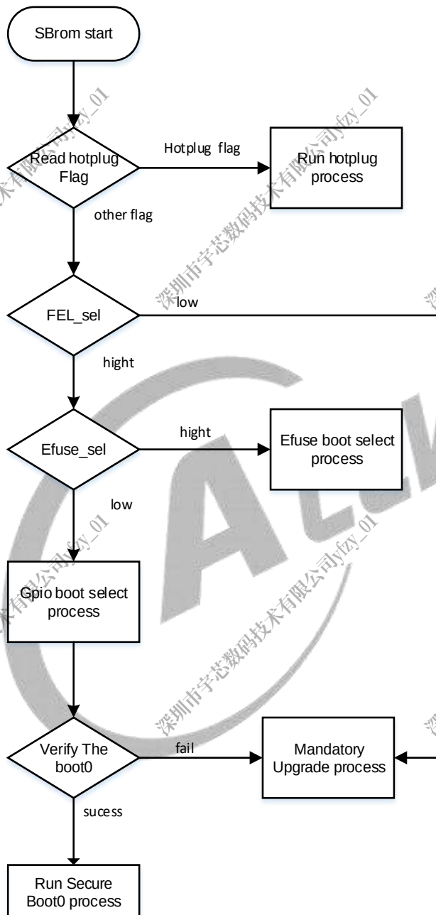
Figure 3-12 Security BROM Process Diagram
