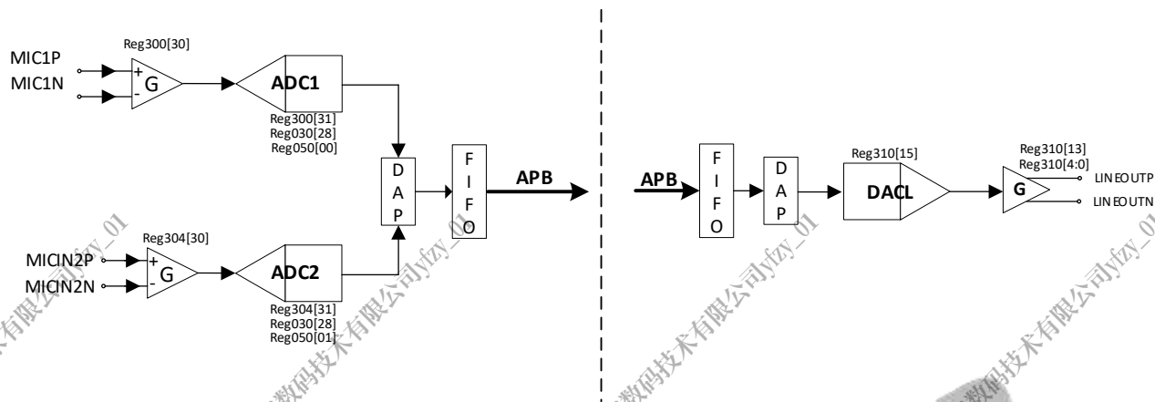
Figure 8-15 Audio Codec Data Path Diagram
