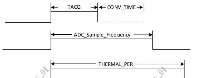
Figure 3-27 Thermal Sensor Timing Requirement
