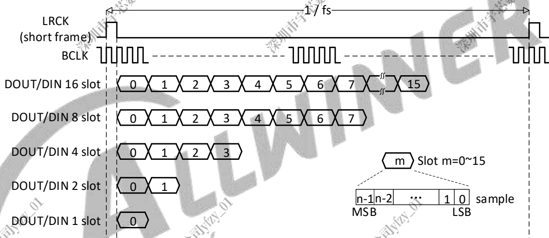
Figure 8-7 PCM Short Frame Mode Timing
