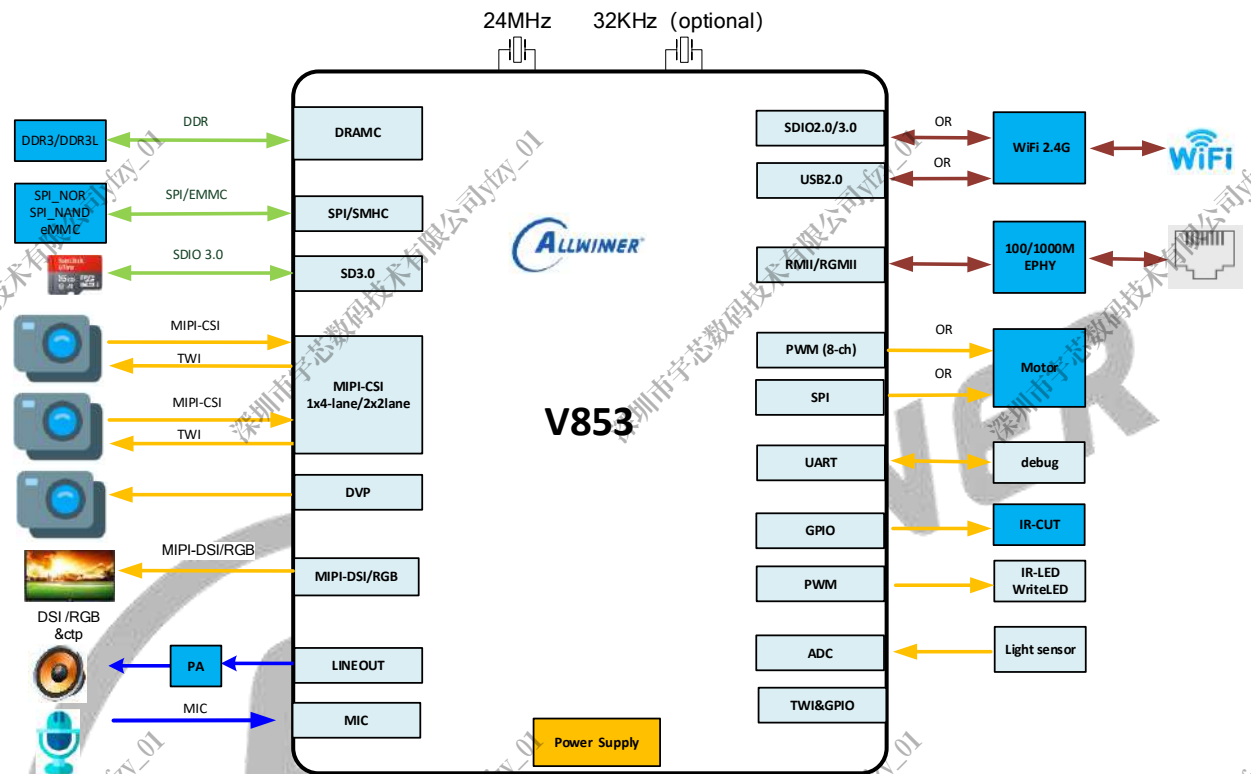
Figure 1-1 V853 AI Vision Solution
