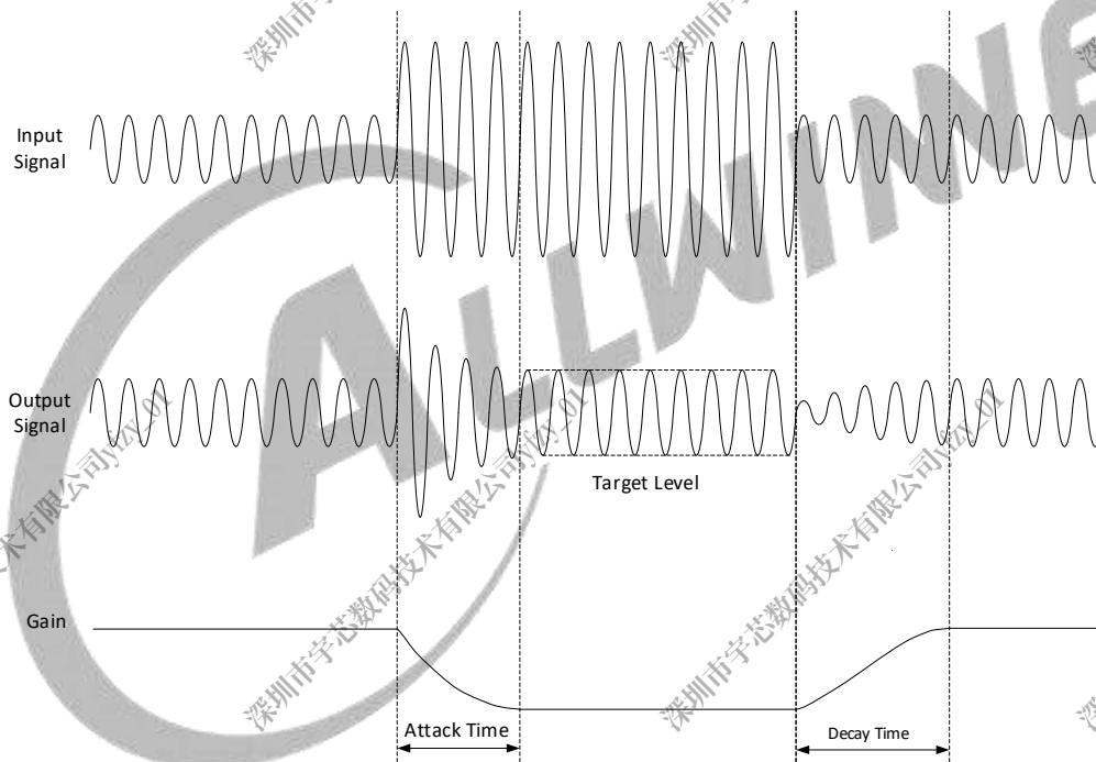
Figure 8-22 Gain Smooth Filter
