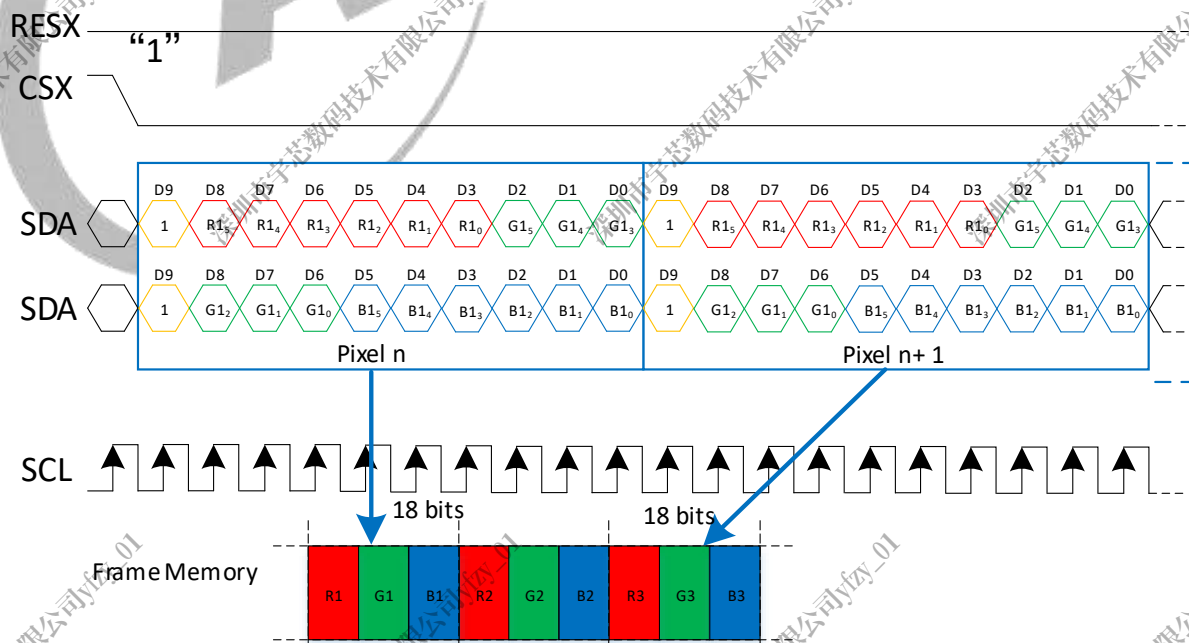
Figure 10-54 RGB666 2 Data Lane Interface Transmit Video Format 0
