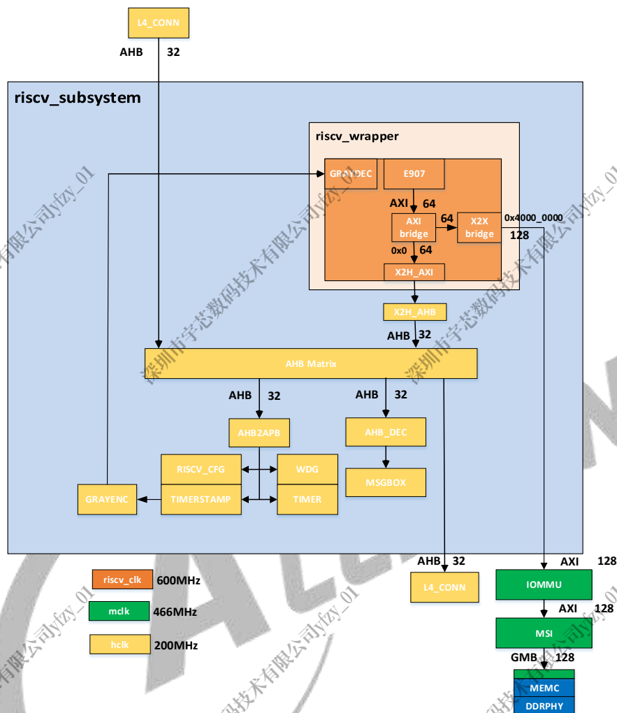
Figure 3-2 RISC-V System Block Diagram
