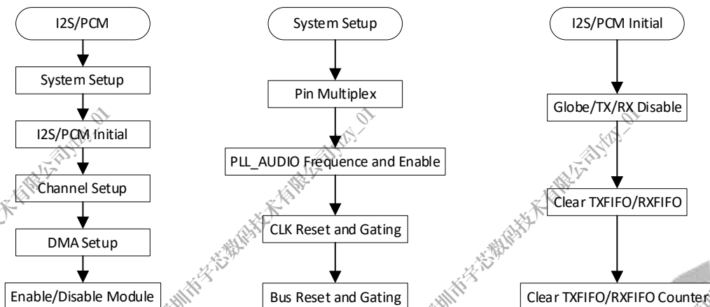
Figure 8-8 I2S/PCM Operation Flow
