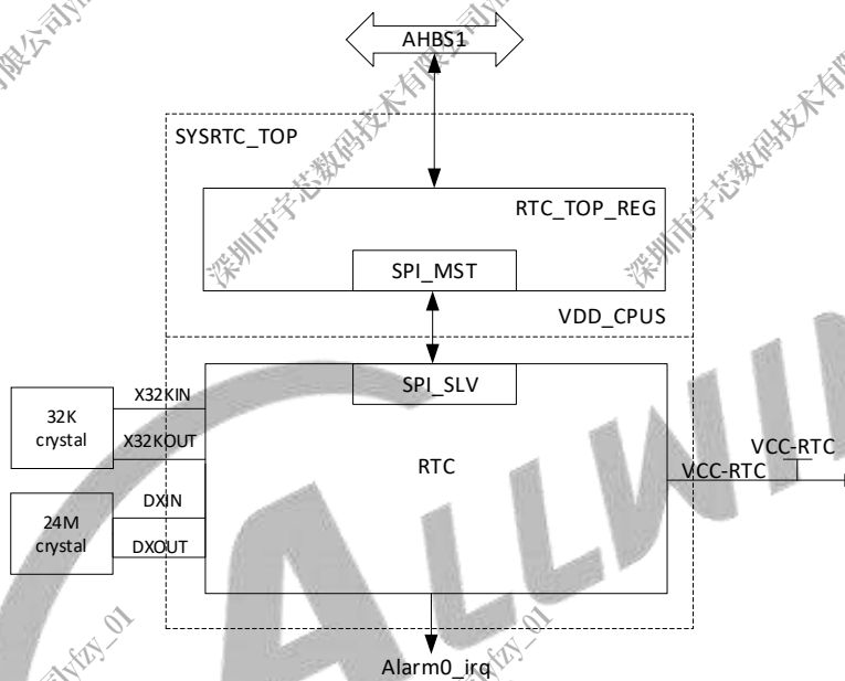
Figure 3-42 RTC Application Diagram
