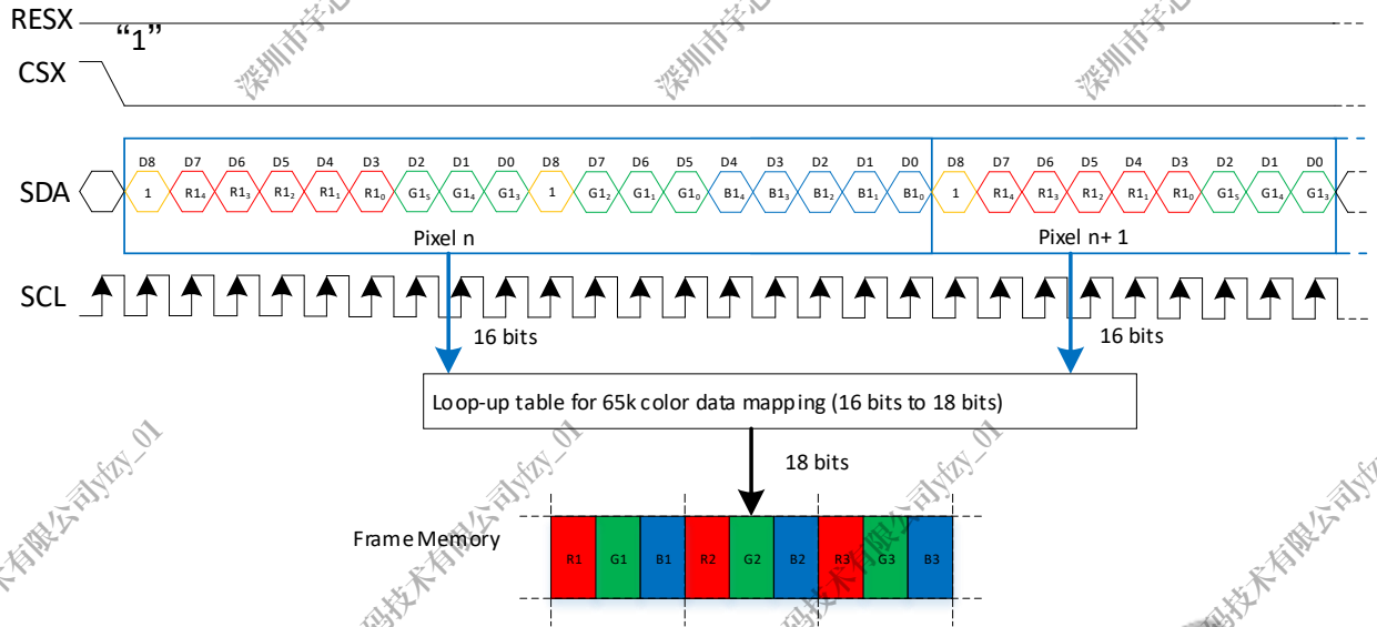
Figure 10-46 RGB565 3-Line Interface Transmit Video Format
