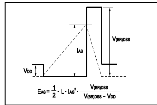
Fig.12 Avalanche Waveform
