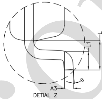
DETAIL Z
