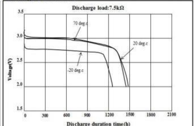
Discharge Characteristics
