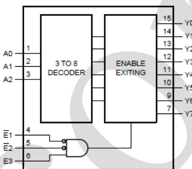
Figure 2. Functional diagram
