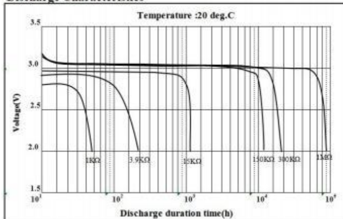
Discharge Characteristics
