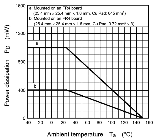
Fig. 8.13 P_D - T_a
