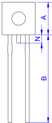
TO-92
